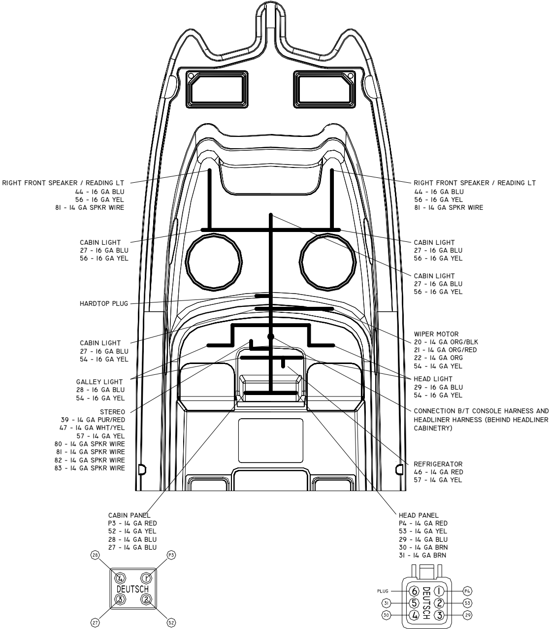
HARDTOP PLUG
